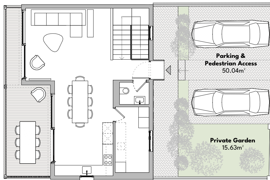
HOUSE + ENTRANCE + PARKING (Entrance Level)
