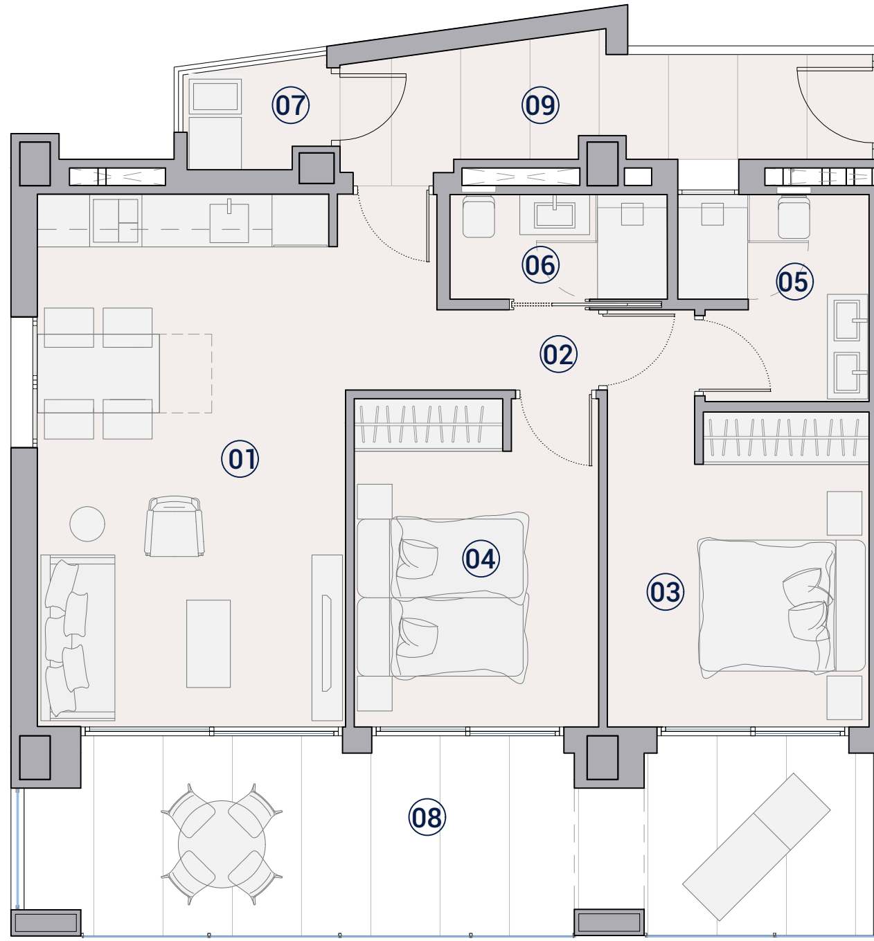
OPC 1 INDOOR LIVING AND OPEN TERRACE
